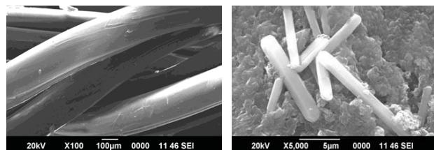
Control PANI treated SEM images of control and PANI treated webbing
