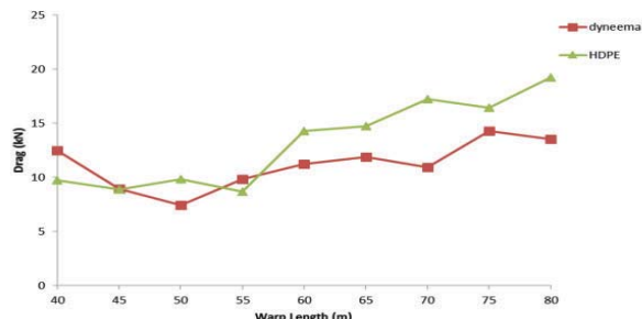
Warp length vs Drag
